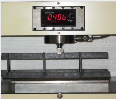
GTI Composite Slab/Beam Bolster 2.0"
